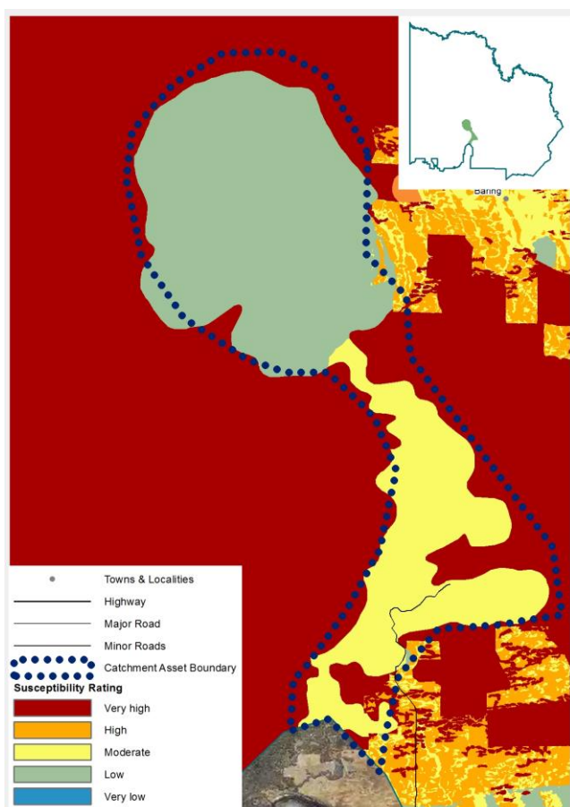
Figure 14: Wind Erosion Susceptibility
