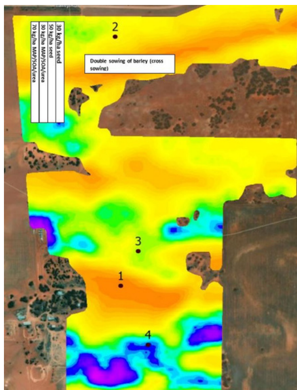
Figure 1. Deep EM38 map with soil test sites, and trial strips on the Charles' property. Red areas are deep sandy soils, generally on hills, blues and purples are the heavier soils, and greens and yellows are the intermediate 'mid-slope' soils.
